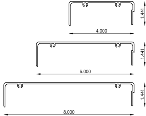
Self Mating Tube (Typ. 3)
