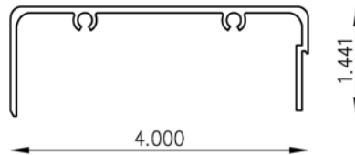
4" Self Mating Tube
