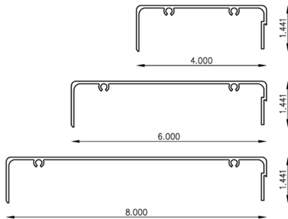
Self Mating Tube (Typ. 3)
